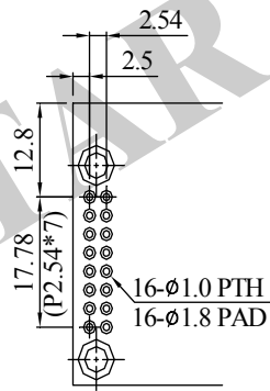
PIN DETAIL SCALE 1/1
