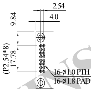
PIN DETAIL
